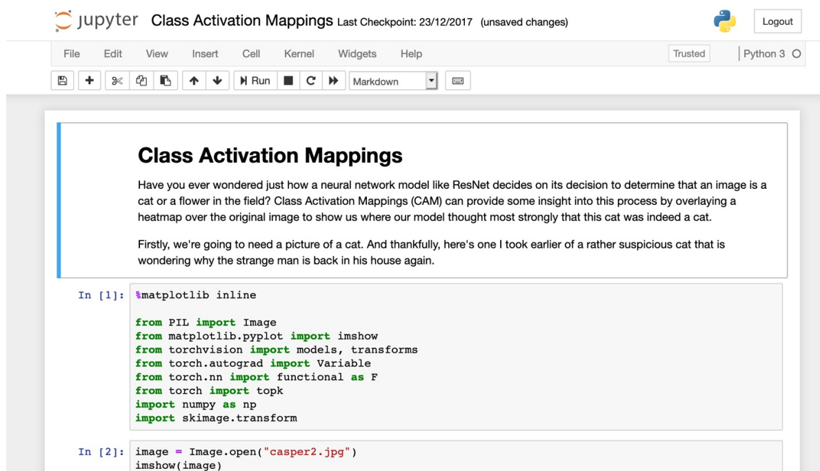
Figure 1-2. Jupyter Notebook
