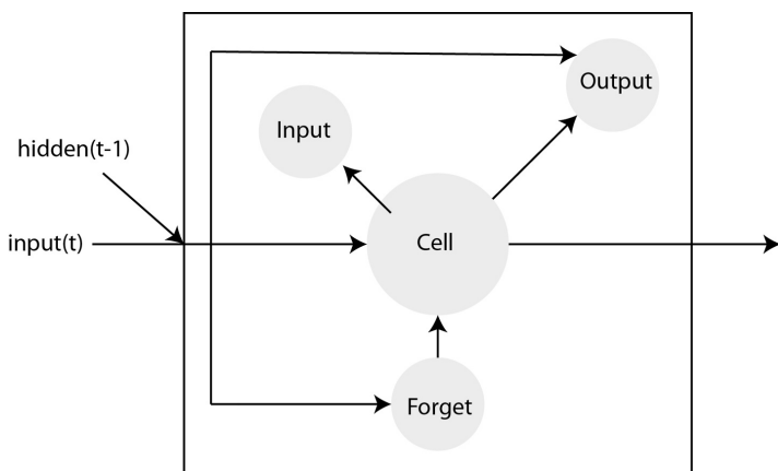
Figure 5-3. An LSTM
